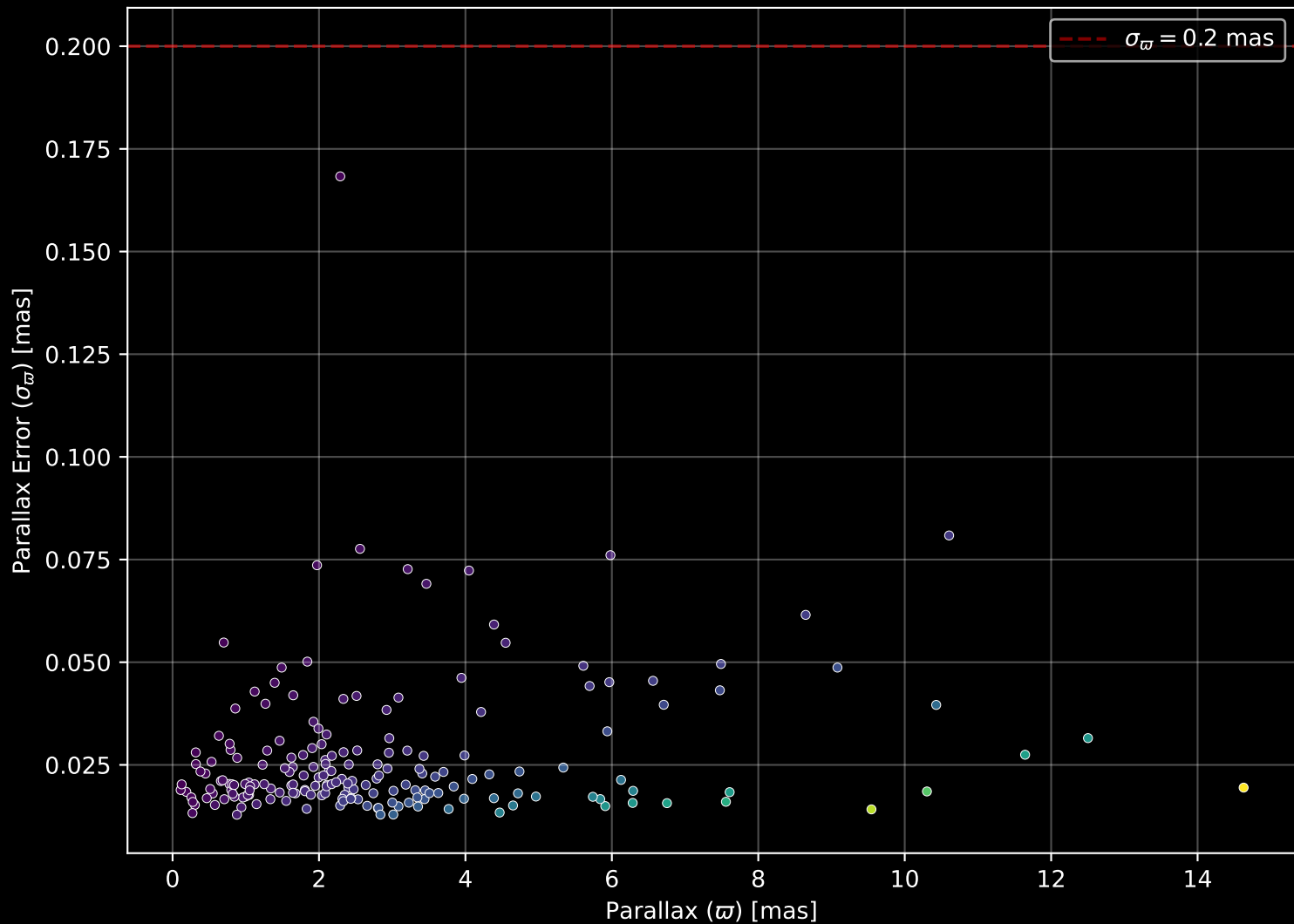
APOGEE DR17 Field: [K2_C5_215+35_btx] Parallax Quality (n= 191)
