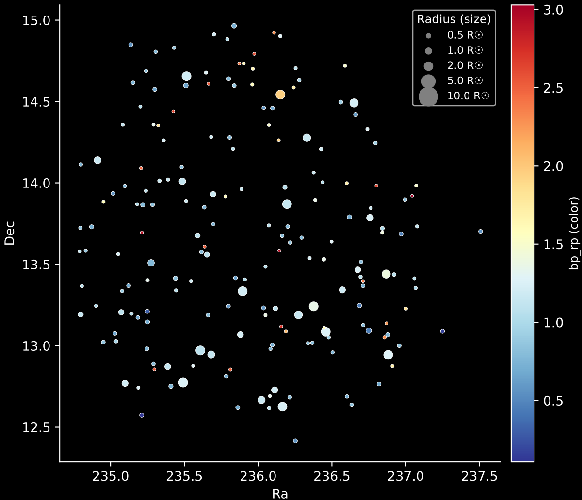
APOGEE DR17 Field: [K2_C5_215+35_btx] Stars: 191
