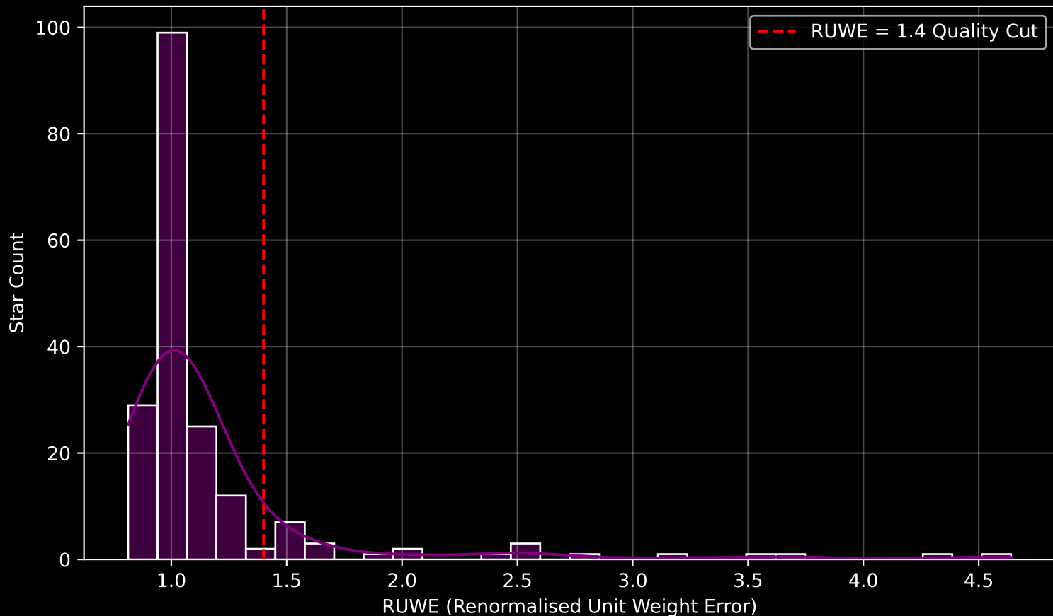
GAPOGEE DR17 Field [K2_C5_215+35_btx] RUWE Distribution (n= 190)
