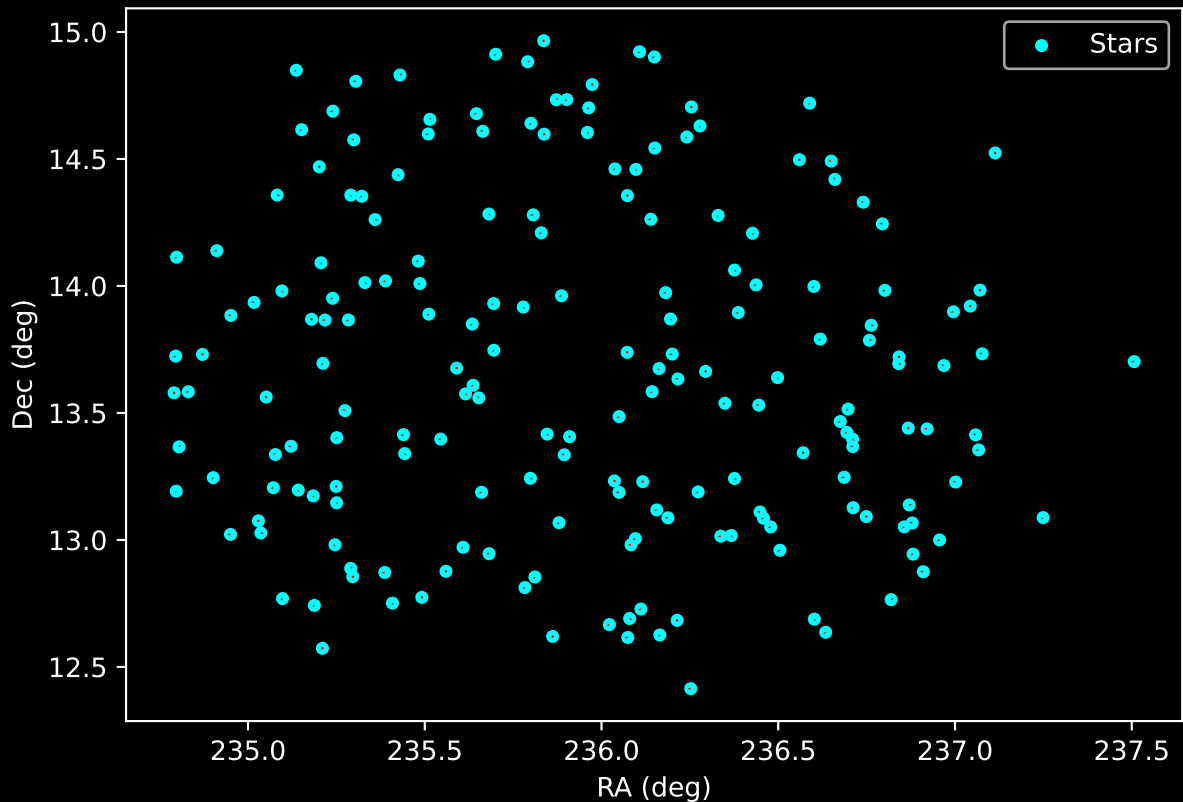
APOGEE DR17 Field: [K2_C5_215+35_btx] Proper Motion Vectors for Gaia Star Field (n= 191)
