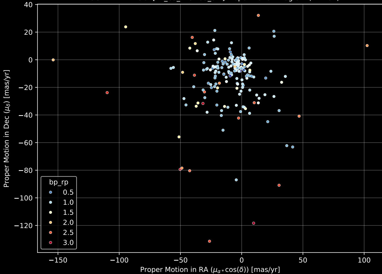
APOGEE DR17 Field: [K2_C5_215+35_btx] Proper Motion Diagram (n= 191)
