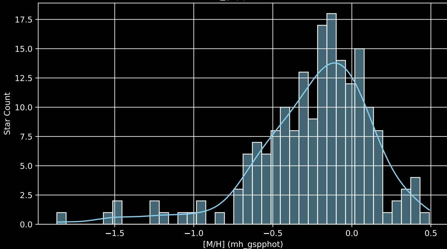
APOGEE DR17 Field: [K2_C5_215+35_btx [M/H] (mh_gspphot) (n= 187)
