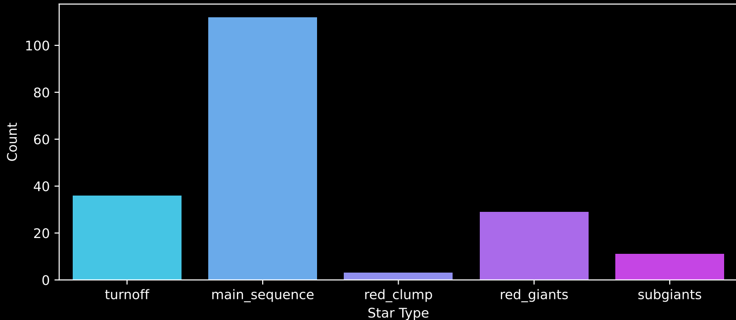
APOGEE DR17 Field: [K2_C5_215+35_btx] Count plot of Star Type
